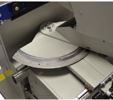
Bohraggregat schwenkbar -65° - 0 - 65°
